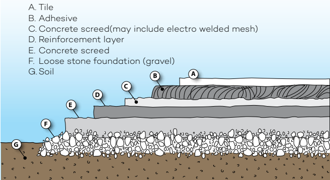
Examples of laying on a soil with adhesive
