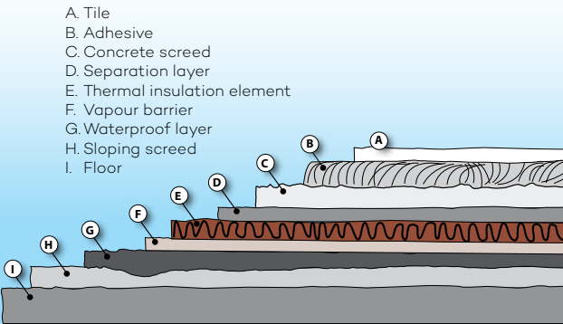
Example of laying on a cement with adhesive
